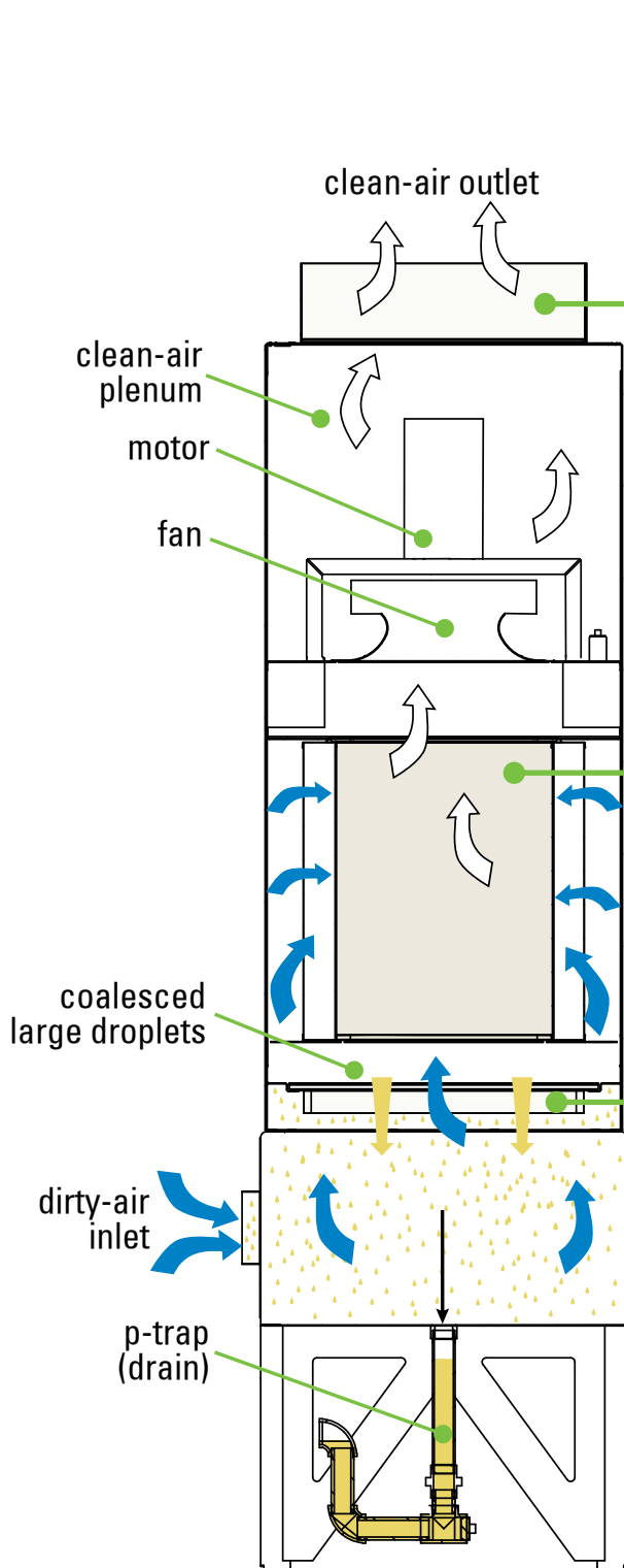
WSO 25-1 with afterfilter
